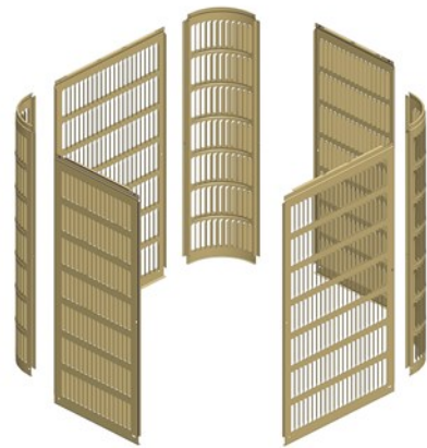
New Independent louver and corner post
